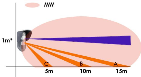
Using the bracket you can change the height of fixing
