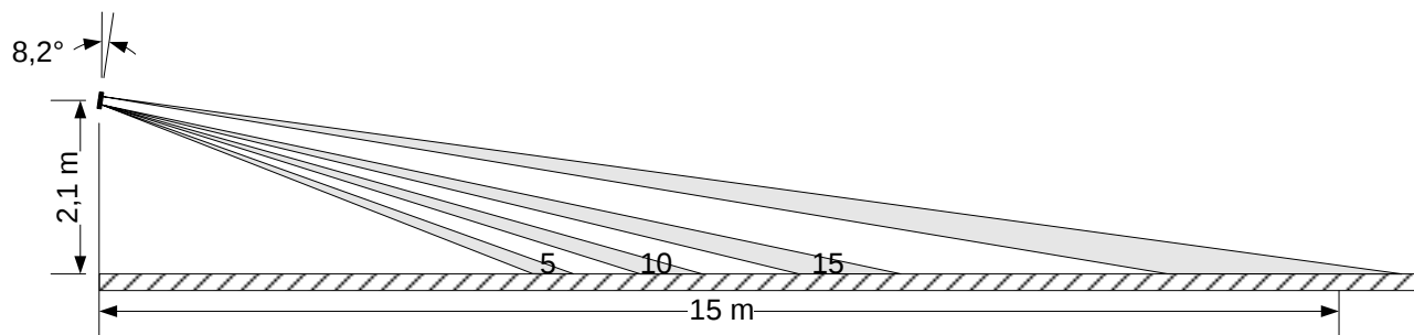
Side view at 2,1 mt mounting with bracket
